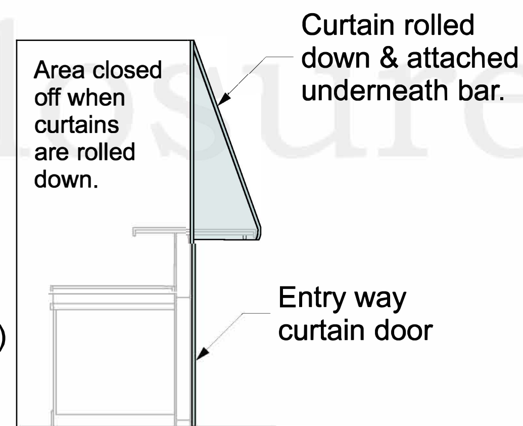
Detail - B
